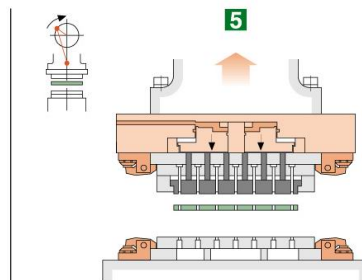
板材脫料 Knock out cycle
