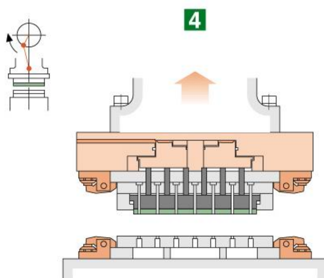
板材提昇 Lifting cycle
